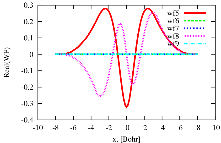
Graphene WaveFunctions@Gamma, slice z=0
