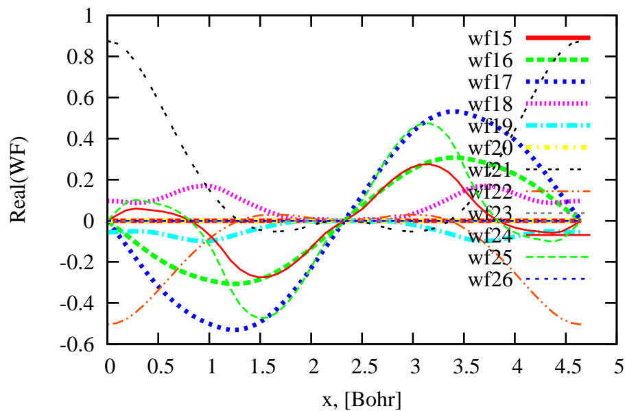
Graphene WaveFunctions@Gamma, slice mgm
