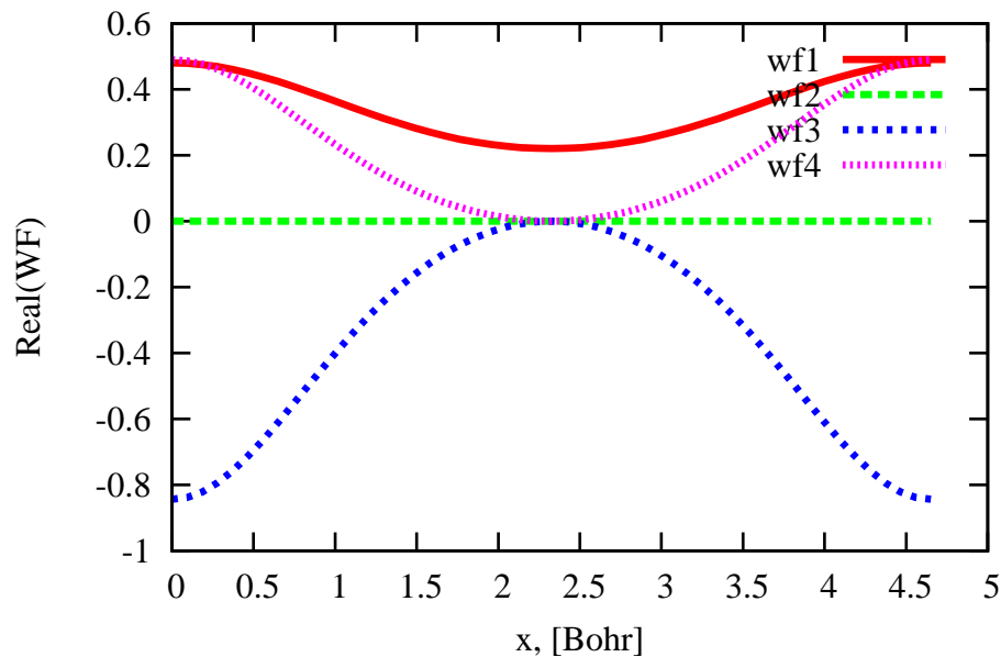
Graphene WaveFunctions@Gamma, slice mgm
