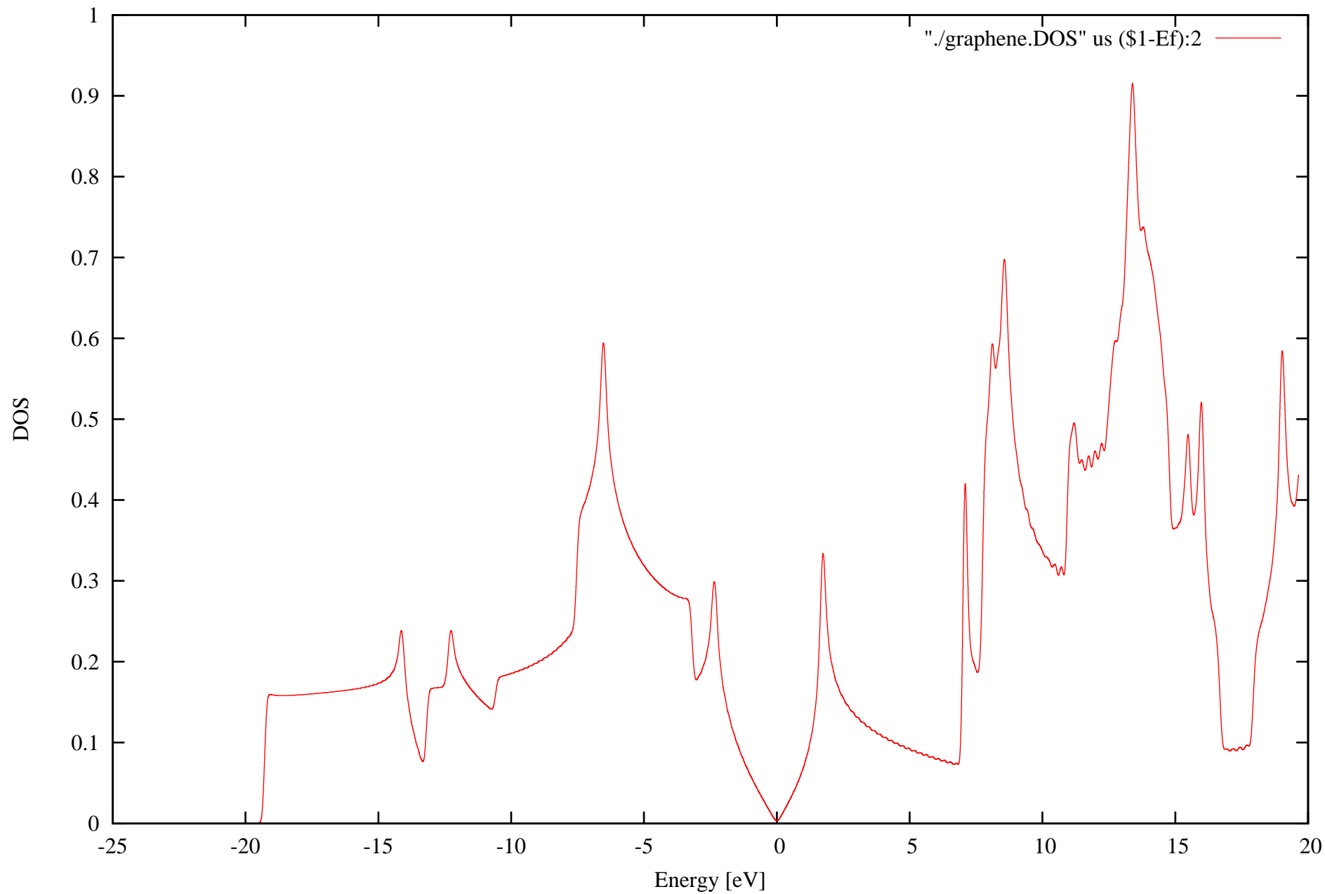
Graphene DOS
