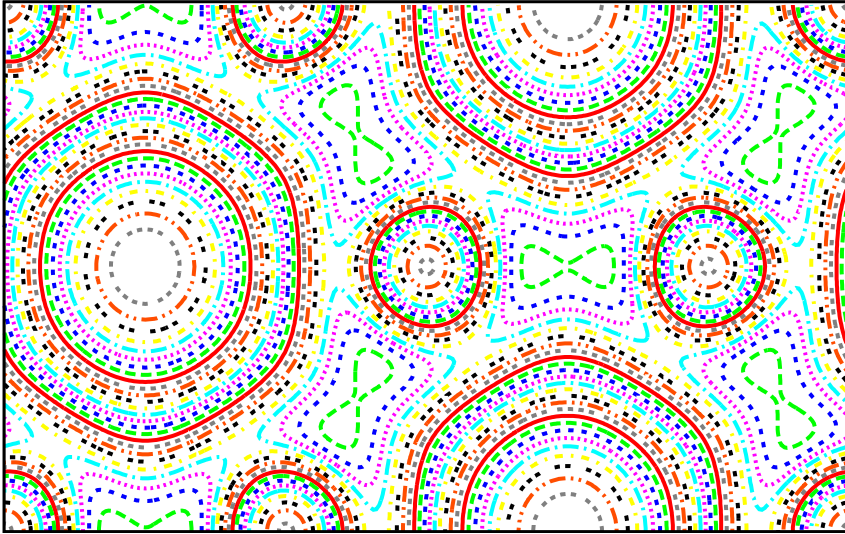
Graphene 2D WF1 @Gamma, slice xky
