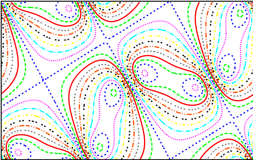
Graphene 2D WF3 @Gamma, slice xky
