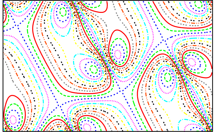
Graphene 2D WF6 @Gamma, slice xky
