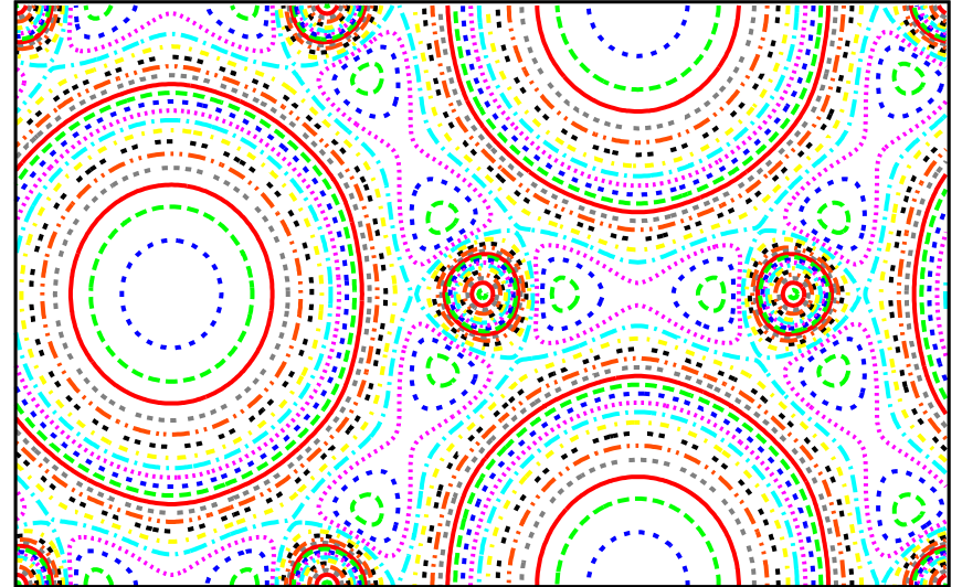
Graphene 2D charge SCF @Gamma, slice xky
