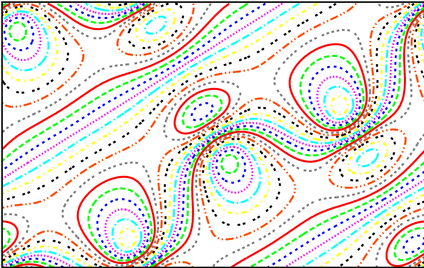
Graphene 2D WF7 @Gamma, slice xky
