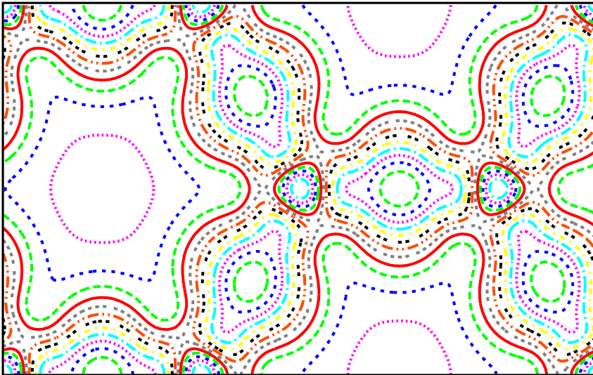
Graphene 2D charge DEL @Gamma, slice xky
