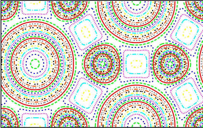
Graphene 2D WF5 @Gamma, slice xky
