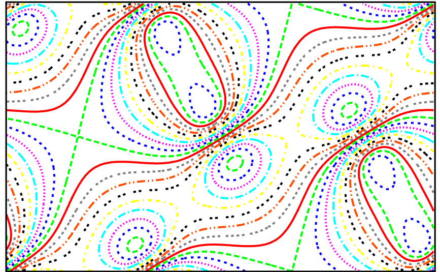
Graphene 2D WF4 @Gamma, slice xky
