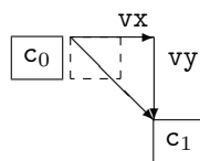
Figure 7.9: Laying out controls using an offset vector.
