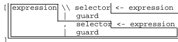
Figure 3.7: Scopes in a list comprehension.
