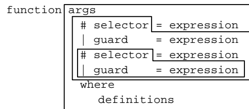
Figure 4.4: Scope of let-before expressions
