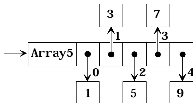
Figure 3.10: Pictorial representation of an array with 5 elements {1,3,5,7,9}.
